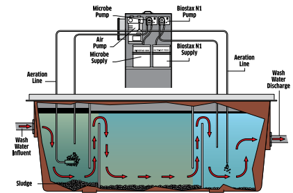
PM-1000D and Collection Pit
